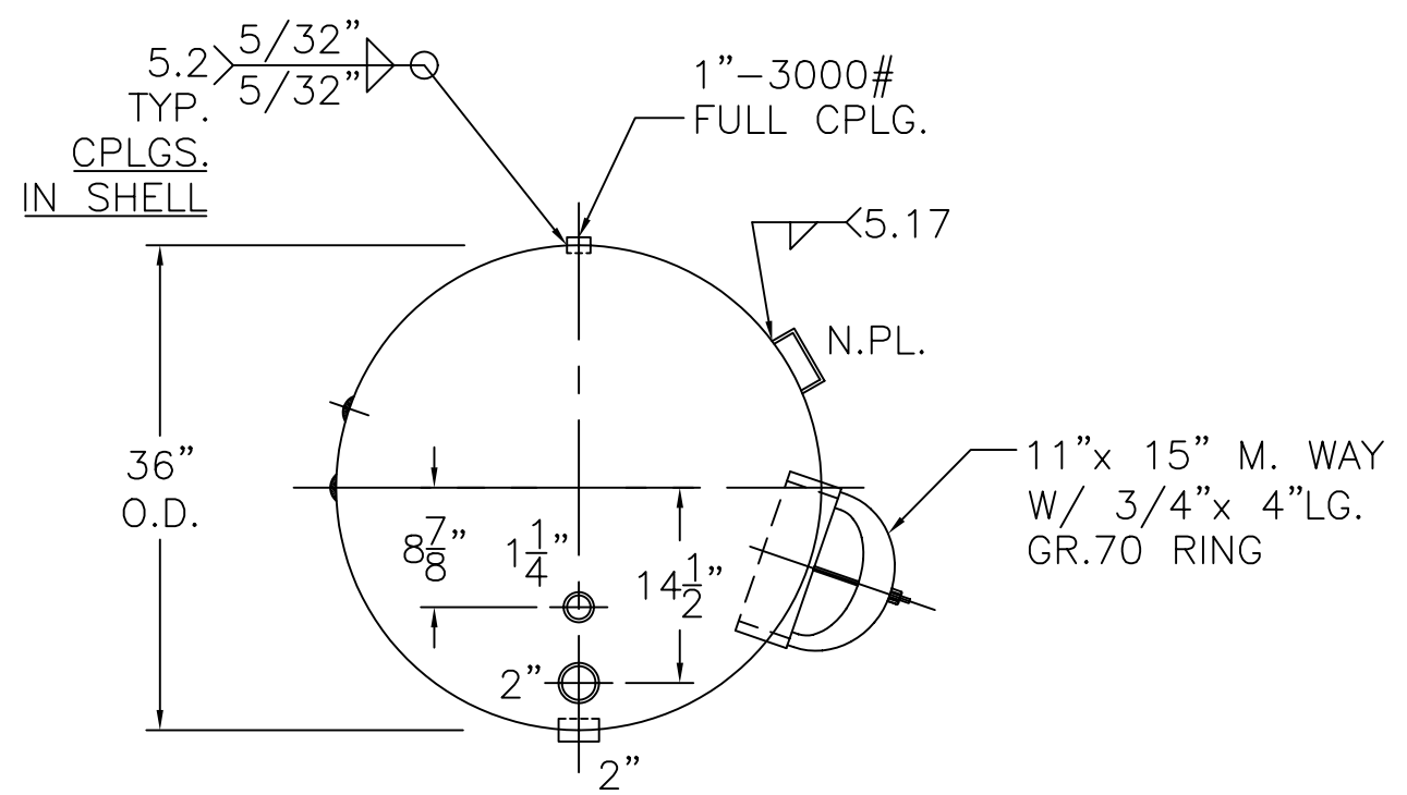
END VIEW W/OUT SUPPORTS
